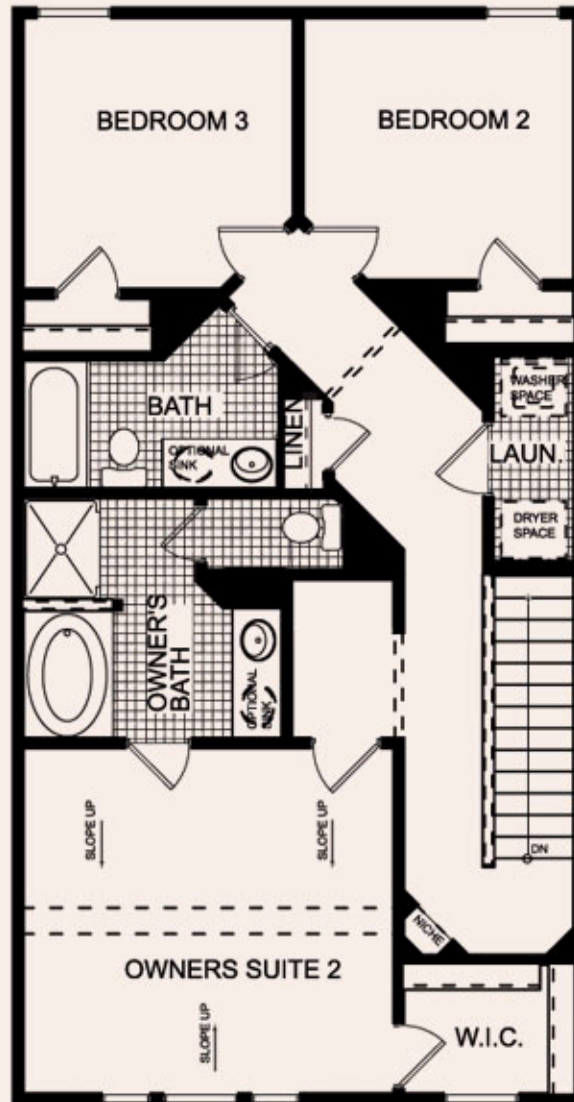
UPPER LEVEL FLOOR PLAN
